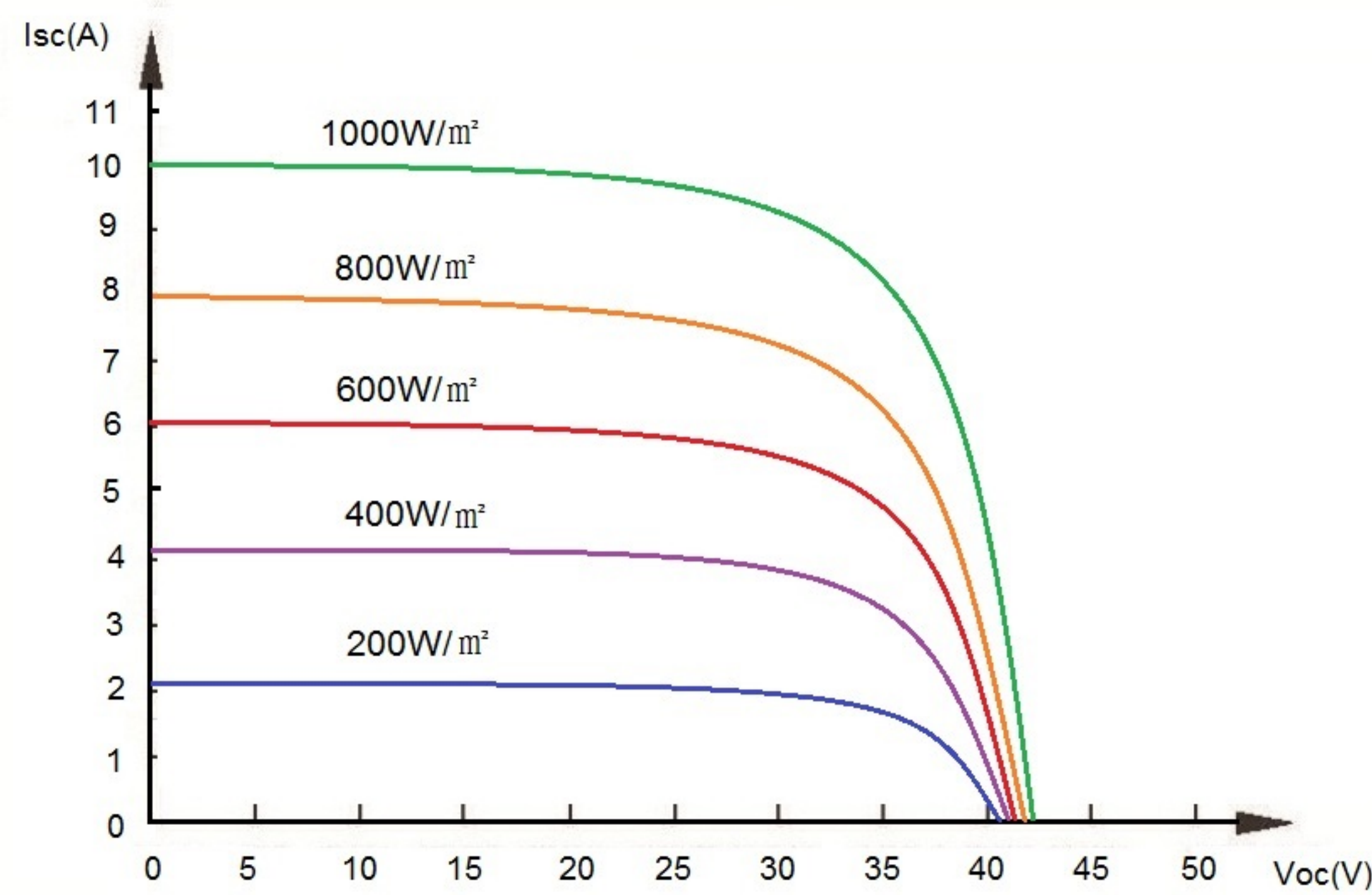
I-V Curves of PV module MS330M-60 at various solar irradiance
