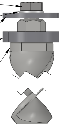
Ground Anchor 50x1000mm, M16 head
